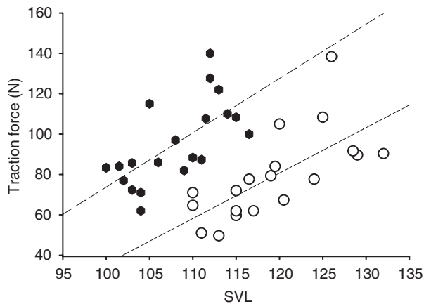
Figure 2 Relationship between maximal contraction strength (N) and snout-vent length of 20 male (●) and 19 female (○) rainbow boas. Each point represents an individual snake.
