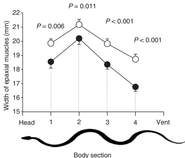
Figure 1 Musculature profiles measured in nine male (●) and eight female (○) rainbow boas with similar body sizes. Dorsal muscle widths (mm) were measured at four equidistant points between the head and the vent (one to four starting from the head). P-values were obtained from ANOVA analysis using musculature width as the dependent variable and sex as the factor.
