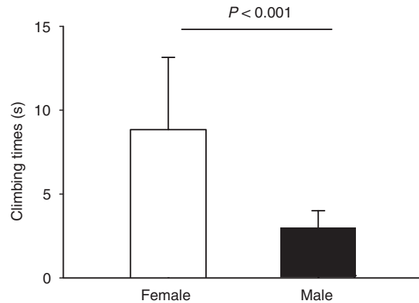
Figure 3 Climbing ability of 20 male (black bars) and 19 female (white bars) rainbow boas. When suspended by the tail, males took less time to reach the hand of the operator than did the females. Error bars represent standard deviation.
