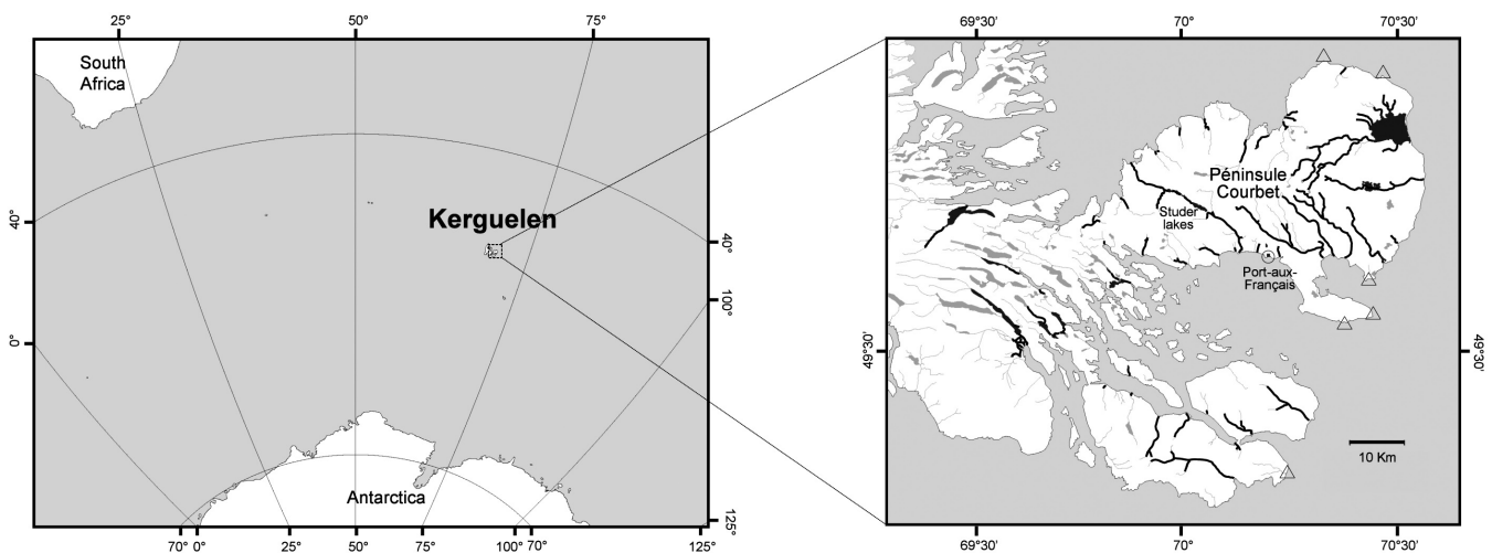
Fig. 1. (a) General location of the Kerguelen Islands in the Southern Ocean. (b) Map of eastern Kerguelen Islands, showing all river systems containing salmonid fish. Port-aux-Français is the French research station. Triangles represent the main known Kerguelen Shag Phalacrocorax verrucosus colonies of 200–2000 breeding pairs. Fish are present mostly on Péninsule Courbet. River systems in grey are free of fish. Systems or river portions in black are populated. The first successful introduction of fish took place in the lakes of the Studer river system, where the first observation was made of a Kerguelen Shag freshwater fishing.
