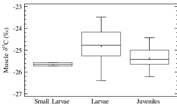
Fig. 4. Carbon isotopic signature of early life stages of P. antarcticum .
