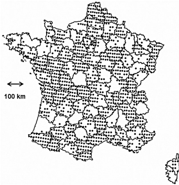
Figure 6 Map of the 1206 sampling quadrats of 5 km × 5 km over France (projection: Lambert azimuthal equal area, ETRS89, EPSG3035). The minimum and maximum distances between observations are, respectively, 15 and 1200 km.
