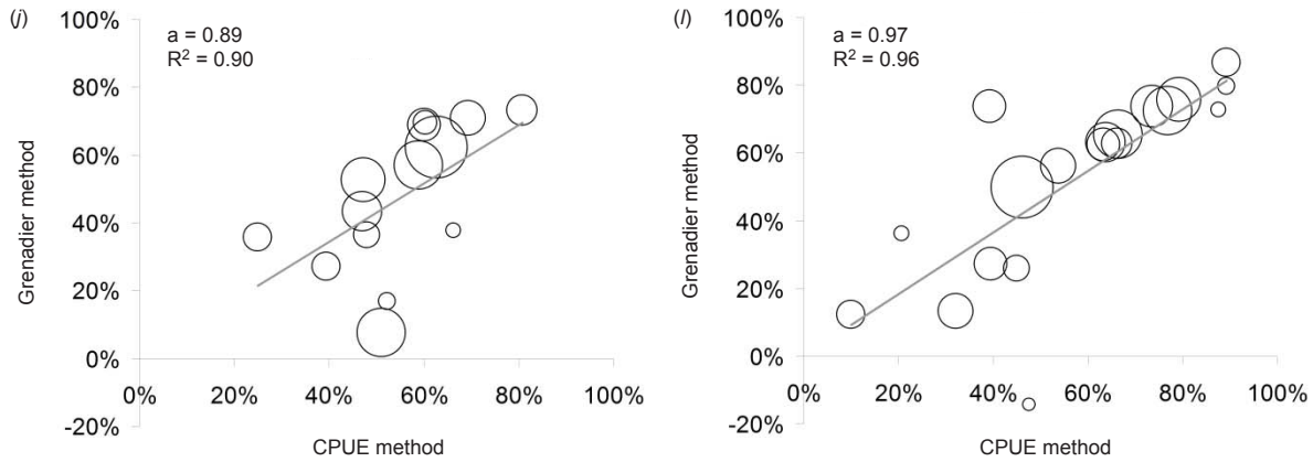
Figure 4: Tests of consistency of the results between the depredation rate estimates provided by method 1 and the depredation rate estimates provided by method 2 in cells c_d and c_g in which data were available for both methods and for killer whales alone (j) and killer and sperm whales combined (l). The regression coefficient (a) and correlation coefficient ( R^2 ) are provided at the top left. The size of circles indicates the amount of toothfish caught on undepredated hooks in each cell (amount ranges from 724 to 10 538 individuals).
