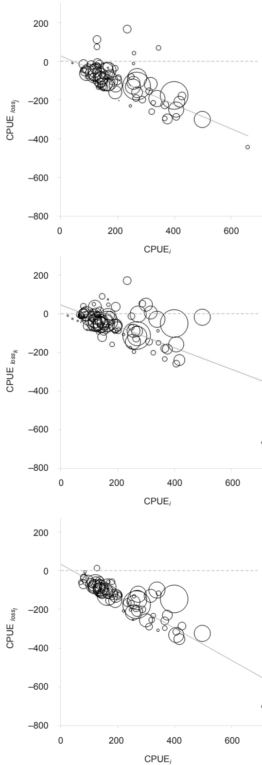
Figure 2: Influence of area richness (Patagonian toothfish CPUE in the absence of odontocete depredation – i ) on the decrease in CPUE caused by depredation (difference of CPUE between non-depredated and depredated hooks – CPUE_{loss} ) in cells c_d . CPUE_{loss} was calculated for hooks that were exposed to depredation by killer whales only ( j – top), sperm whales only ( k – centre) and both species co-occurring ( l – bottom). Linear regression curves are depicted (dark line – R^2 = 0.53; 0.44; 0.88 for j, k and l respectively). The size of the circles indicates the amount of toothfish caught on undepredated hooks in each cell c_d , the largest circle represents 108 tonnes.
