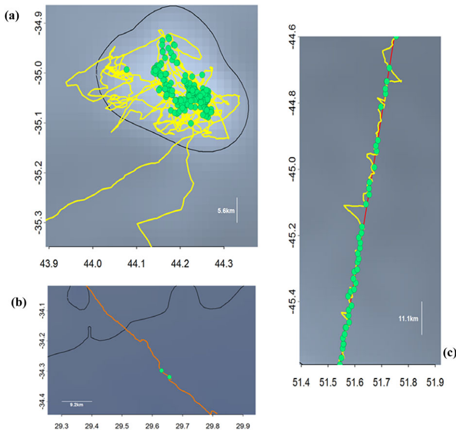
Figure 2. Movement pattern of wandering albatrosses equipped with biologging devices that detect radar emissions and record the position of boats (green dots) and seabirds (yellow and orange lines): (a) attending behavior behind a Japanese fishing vessel (identity determined from Globalfishingwatch.org), (b) fly-past behavior, and (c) follow behavior (red lines, track of vessel).
