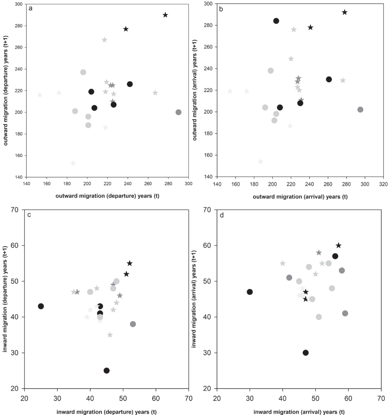
Fig. 4. Migration characteristics of Grey Petrels tracked from the Kerguelen Islands in consecutive years (2007–2012) to non-breeding areas: a) date of departure from breeding the colony (spring), b) date of arrival at the first non-breeding area, c) date of departure from the last non-breeding area, and d) date of arrival at the breeding colony (autumn). The timing of migration is shown in Julian days. Dates during year (t+1) on the y-axis are plotted in relation to dates during year (t) on the x-axis (symbols represent different individuals).
