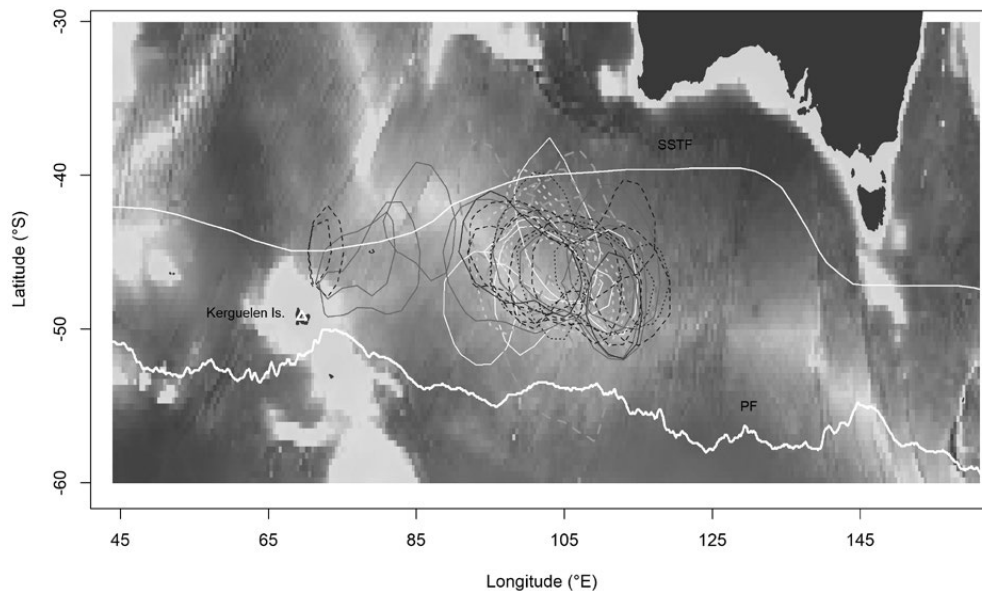
Fig. 1. Distribution of Kerguelen-breeding Grey Petrels carrying loggers for two or more successive non-breeding periods (colored by individual; seven individuals) in the southern Indian Ocean, 2007–2012. UD is the mean utilization distribution estimated using all locations recorded for each individual track in each year (50 % UD). Oceanographic frontal structures (grey lines)—the South Subtropical Front (SSTF) and Polar Front (PF) (Belkin and Gordon 1996; Sokolov and Rintoul 2009)—are shown. Bathymetry is represented in the background.
