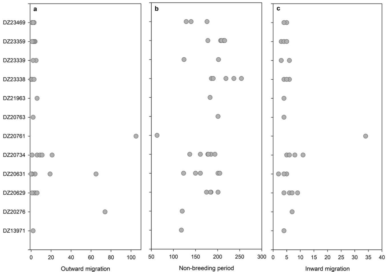
Fig. 3. Individual differences in the total number of days spent by Grey Petrels in a) outward migration, b) the non-breeding period, and c) inward migration. Codes on the y-axis correspond to ring numbers.
