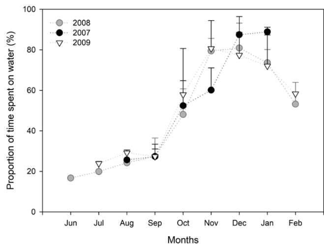
Fig. 6. Activity patterns of adult Grey Petrels (average daily proportion of time spent on the water with time) during the non-breeding period.
