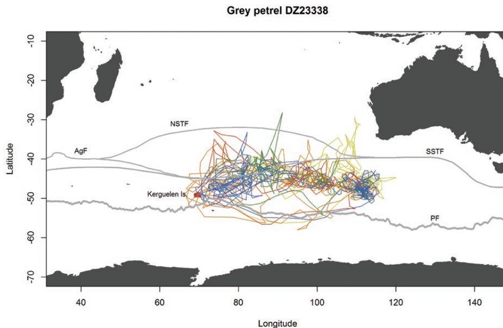
Fig. 2. Example tracks of one Grey Petrel from the Kerguelen Islands (red triangle) during the non-breeding period in five consecutive years (1st year: yellow, 2nd year: orange, 3rd: red, 4th: green, 5th year: blue). Oceanographic frontal structures are depicted as in Fig. 1.
