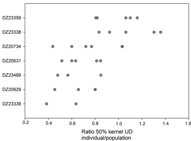
Fig. 5. Ratio between individual and population 50 % utilization distribution kernels of Grey Petrels tracked from the Kerguelen Islands during the non-breeding period in consecutive years, 2007–2012.
